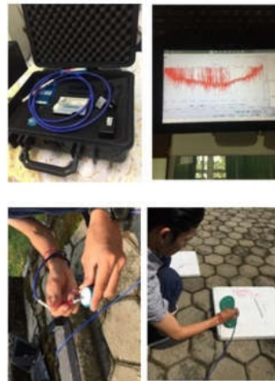
Figure 4. Spectral measurement of plastic debris using Ocean Optics USB 4000.
